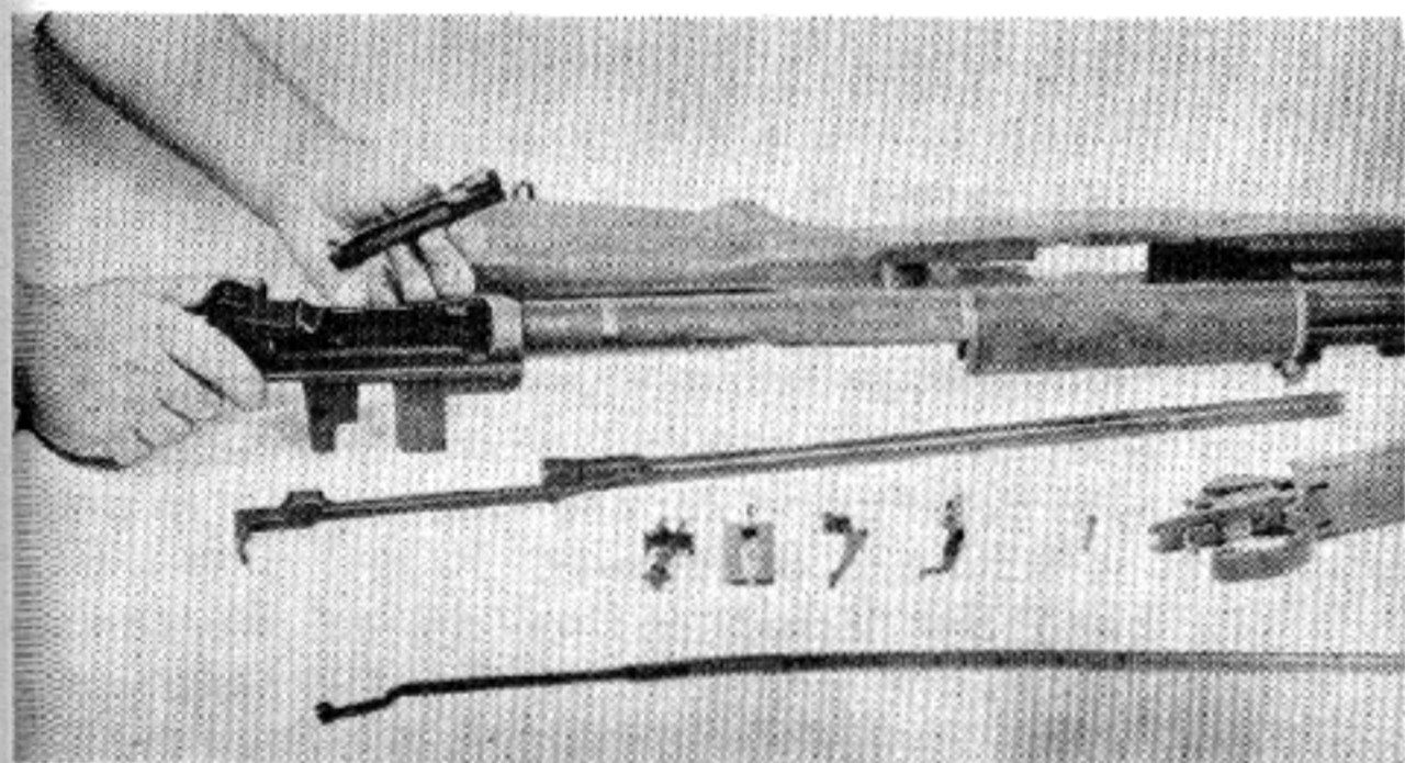
7. Slide the bolt from the rear to the front by pushing the operating lug on it, and lift it out to the right front with a slight twisting motion.
