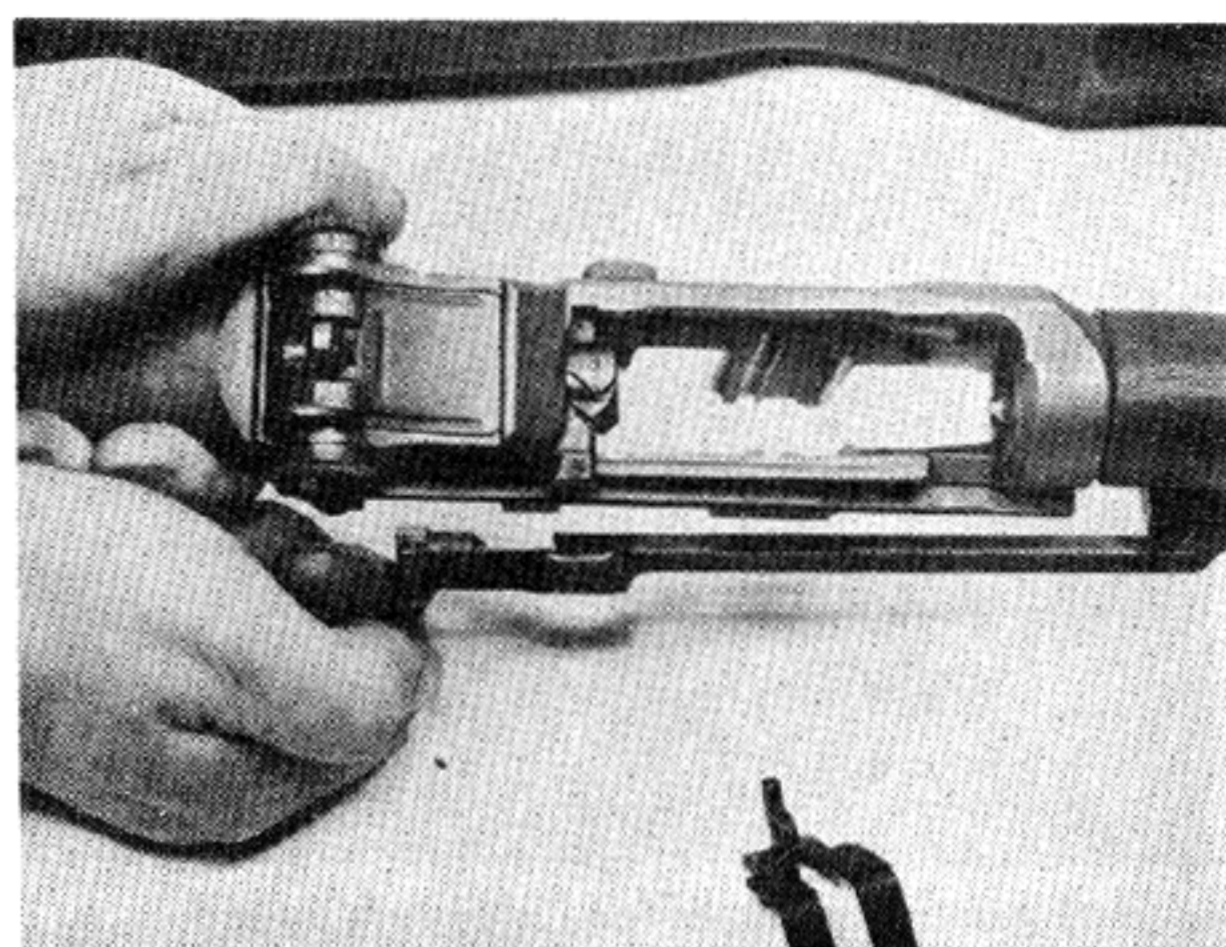
6. Holding barrel and receiver assembly with left hand, grasp the operating rod handle with right hand and move it slowly to the rear, meanwhile pulling the rod handle up and away from the receiver. (This disengages operating rod from bolt, when the lug on the operating rod slides into the dismount notch of the operating rod guide groove.) When operating rod is disengaged pull it down and back and withdraw it. (Note that the operating rod is bent. This is intentional. Do not attempt to straighten it.)
