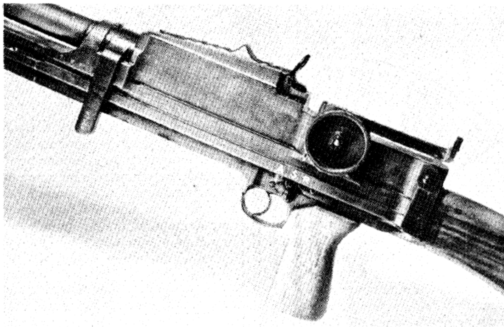
Showing Change Lever for Safe, Automatic, or Single Shot Fire
