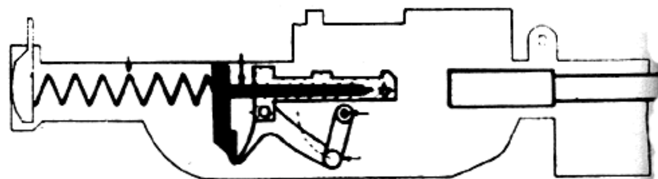
Hesitation Position of Parts
