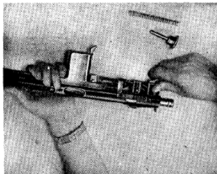
5. Withdraw Hammer Spring. Pull Trigger and let Hammer Slide out.
