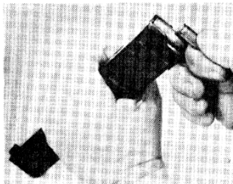
2. To Load Magazine: Hold in left hand. Rest on a solid surface or hold base against hip. Press Cartridge down on front end of Magazine Follower. Slide in under curved lips of Magazine. Repeat until Magazine is filled.
