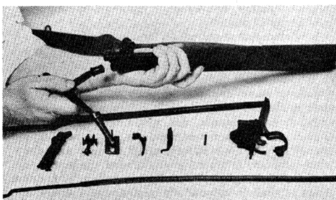
3. The combination tool must be used on this type to unscrew the gas cylinder lock screw.
