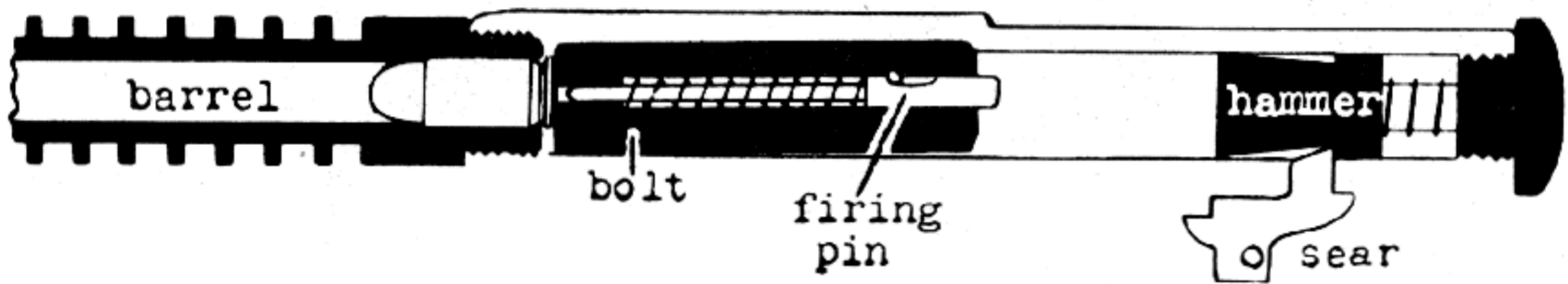
Closed Breech: Example, Reising Submachine Gun
