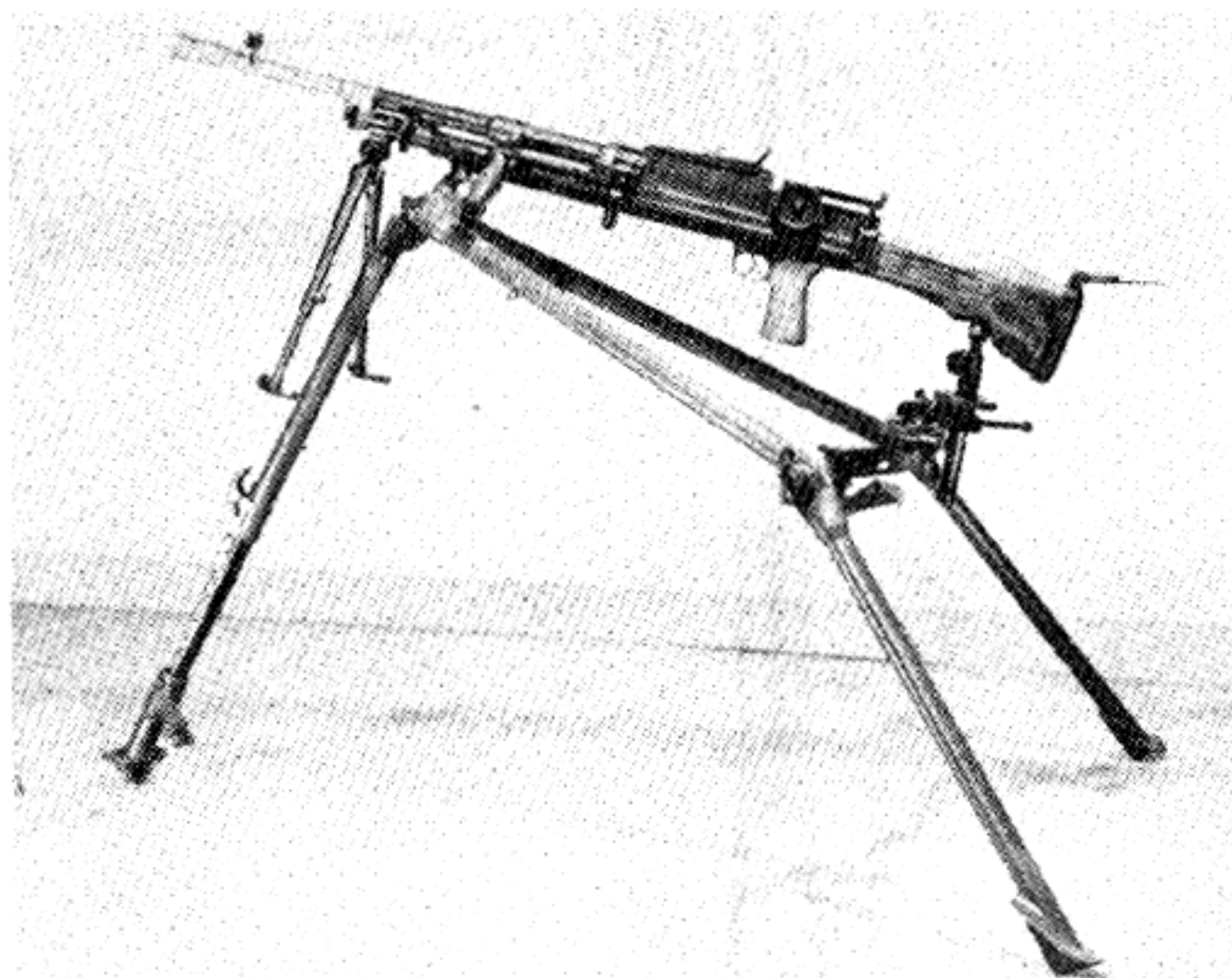
Showing Details of Tripod Mount
