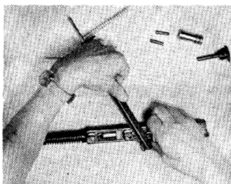
2. Lift ends of Connector and Disconnector and twist Action Bar in under ends of Connector and Disconnector.
