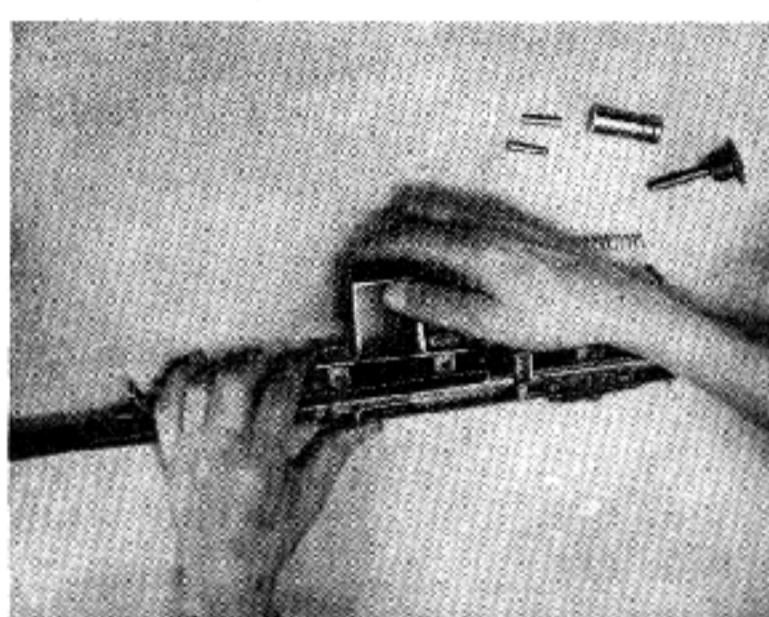
5. Replace the Magazine Guide.
