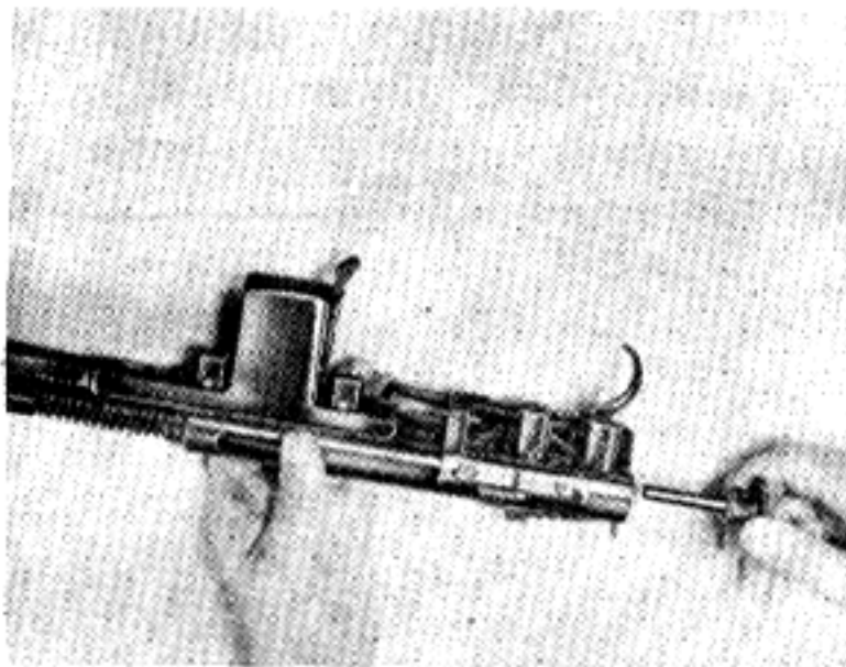
4. (a) Pull Trigger to release tension of Hammer Spring. (b) Unscrew Bumper Plug.
