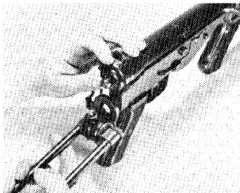
2. With the left thumb press in on the head of the spring tube protruding through the back of the gun. With the right hand
