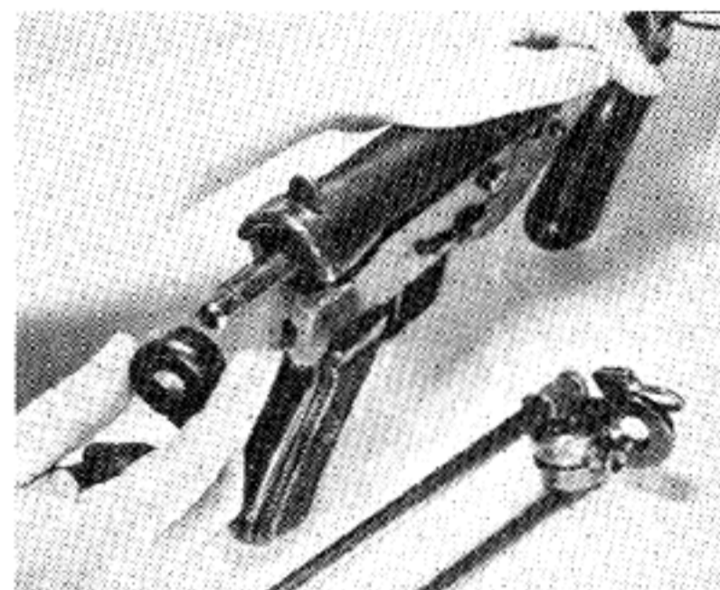
grasp the stock firmly and slide it down out of its locking groove in the rear of the receiver.
