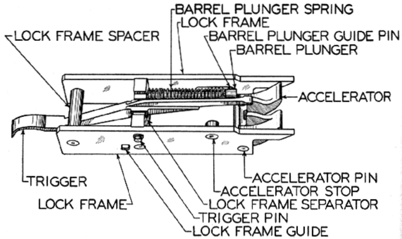
Lock-Frame Assembly
