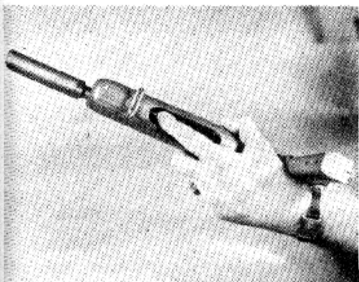
4. To Cock Gun and Load Firing Chamber: With forefinger of left hand, pull back Fingerpiece of the Action Bar as far as it will go. This will (a) Compress the Action Bar Spring. (b) Push back the Bolt. (c) Cock the firing mechanism. (d) Permit Magazine Spring to push top Cartridge in Magazine up into line with the Feed Rib on bottom of Bolt.
