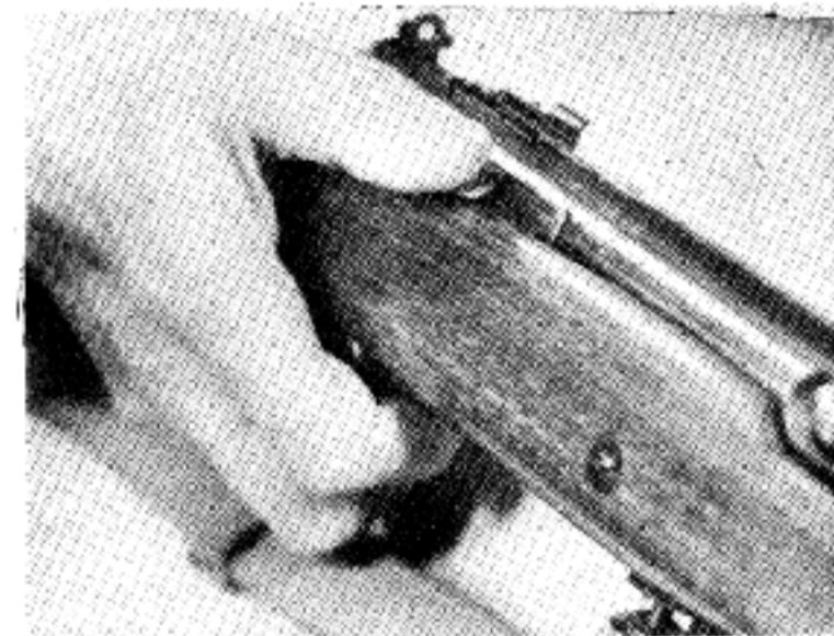
6. To Set Selector: (a) If weapon is not to be used at once, set Selector on "S" (Safe). It cannot be fired in this position. (b) For all normal use, set on "S.A." (Semi-Automatic). It will now fire, eject and reload, one shot for each press of the Trigger. (c) For emergency fire under unusually dangerous conditions, set on "F.A." (Full Automatic). Gun will fire as long as Trigger is held and Magazine contains any Cartridges.
