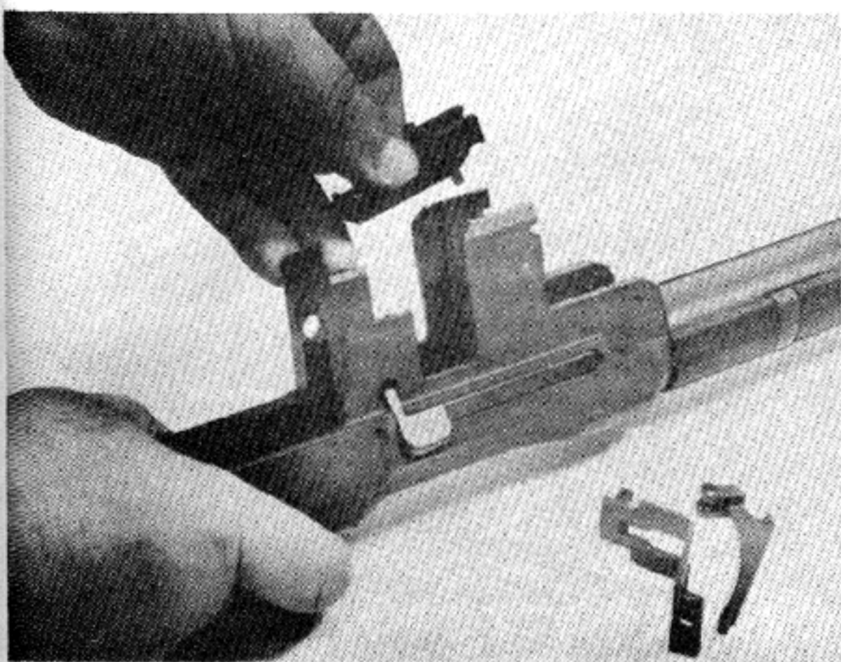
5. Lift out follower with its slide attached (do not separate follower from slide.)
