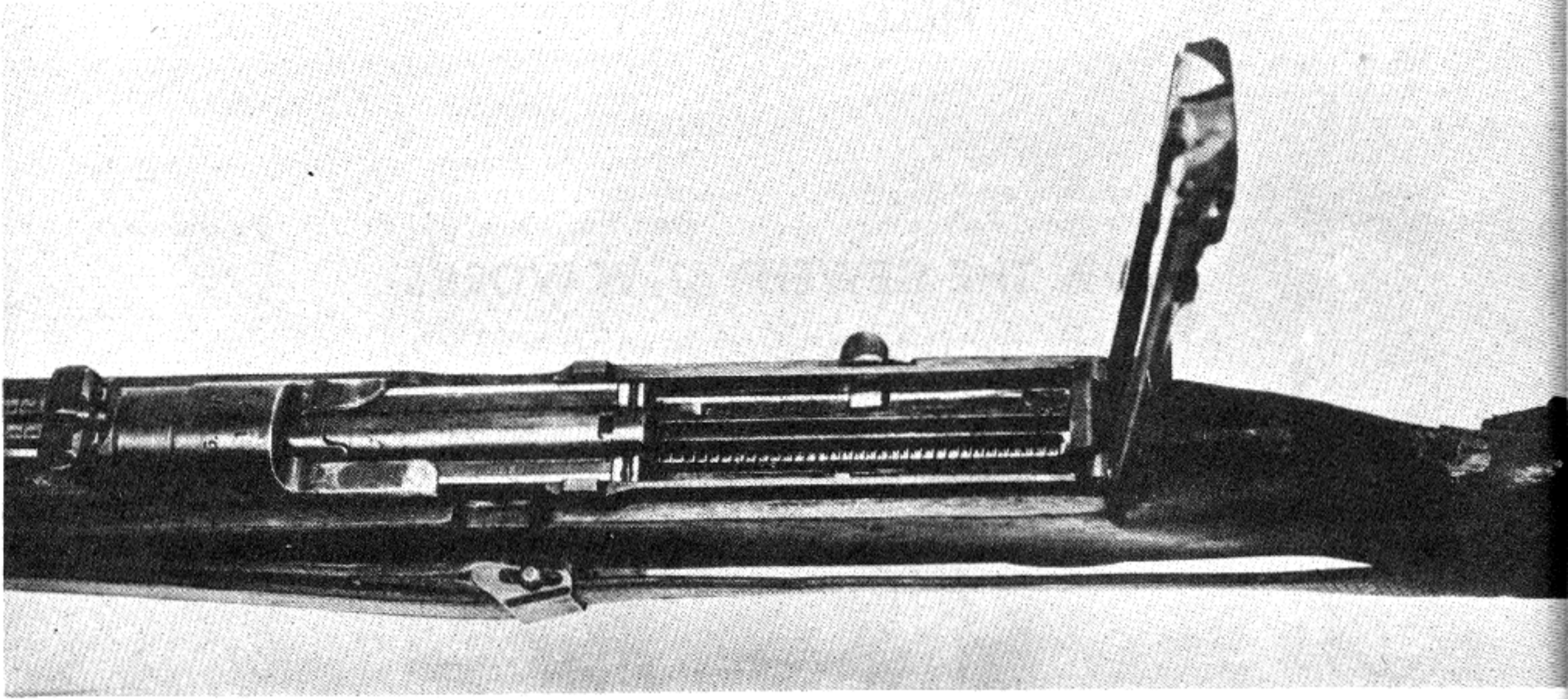
Bolt Cover open, Showing Detail of Bolt and Recoil Spring.
