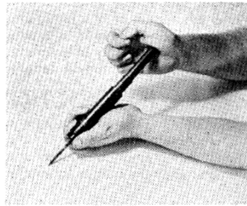
2. Recoil spring housing, showing firing pin and telescoping of tube.
