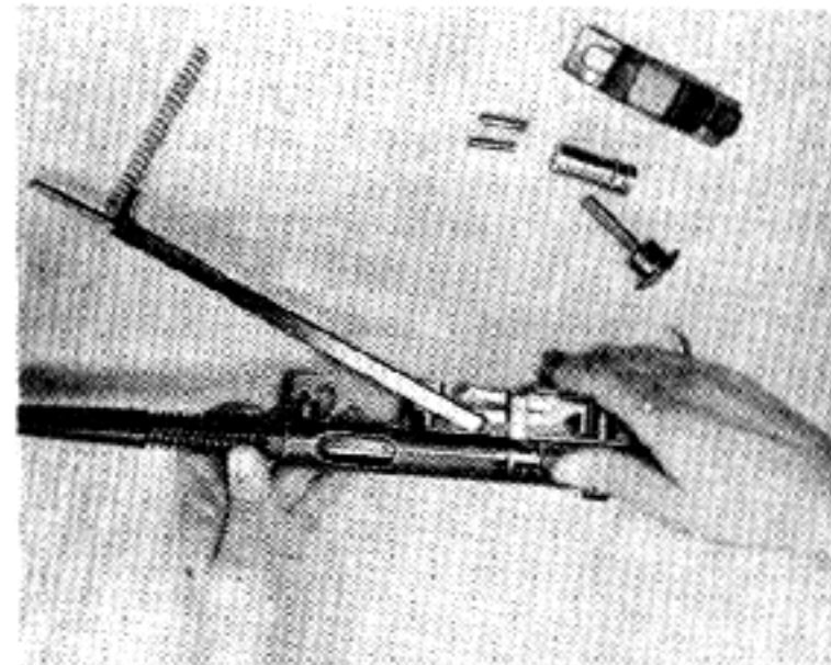
8. With forefinger of right hand, hold up ends of Connector and Disconnecter. With left hand lift forward end of Action Bar to 90 degree angle.
