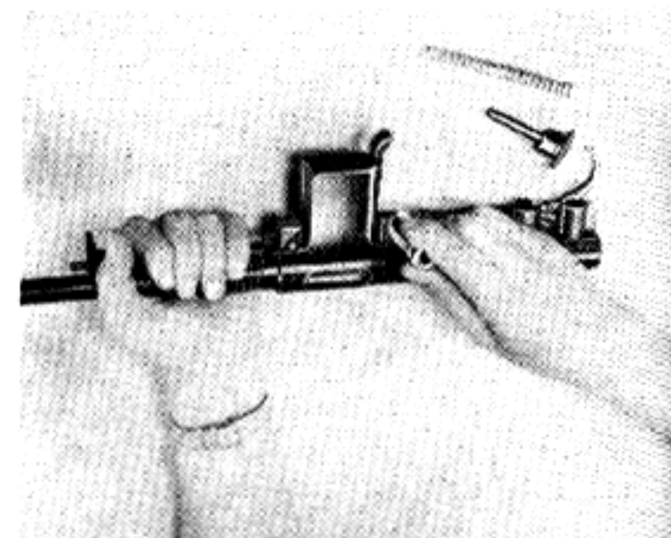
6. (a) Push out the tapered magazine Guide Pins. If they are tight, drive them out with the Gun Hammer as shown above. (b) Remove Magazine Guide.
