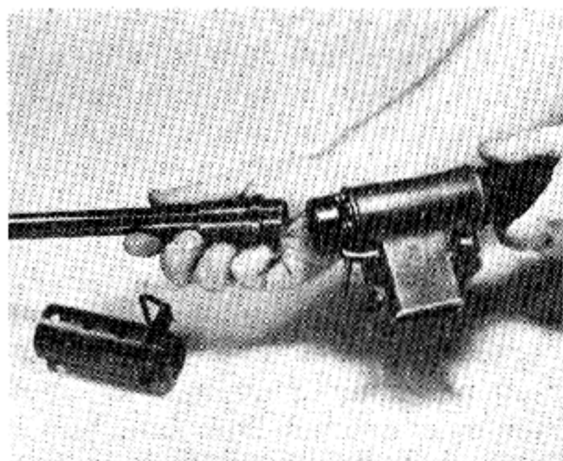
7. Pull the barrel nut and casing forward out of the receiver. Pull barrel straight forward out of the receiver.
