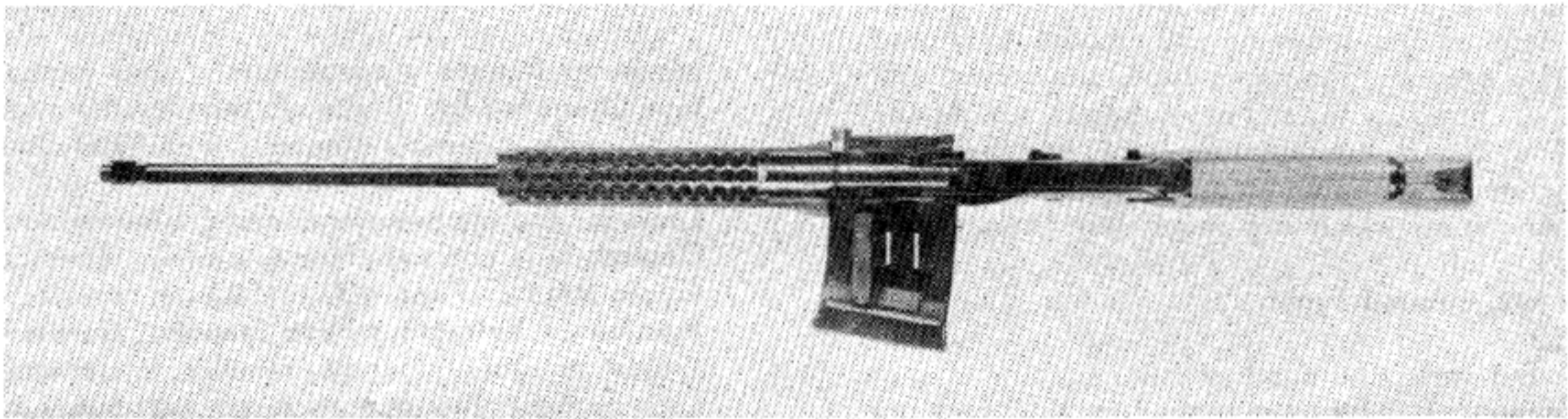
View Showing Magazine, Catch, and Bolt Handle
