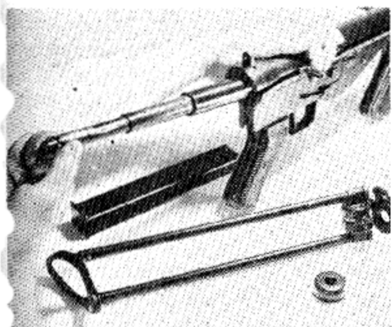
4. Pull back the cocking handle which will bring the recoil and buffer spring tube back and pull the telescoping tube out of the receiver.
