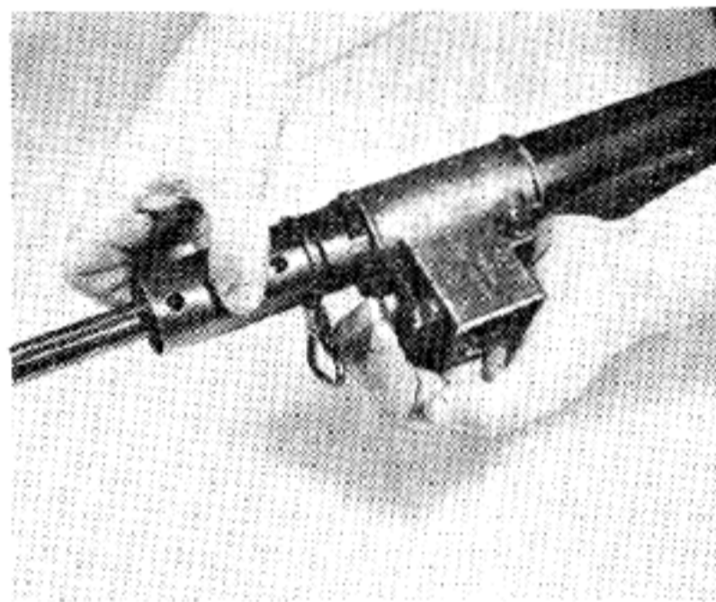
6. With the fingers of the left hand, pull back the barrel nut catch against its spring tension (It is at the front end of the magazine housing on the left side of the gun) and with the right hand unscrew the barrel casing and barrel nut to the right.
