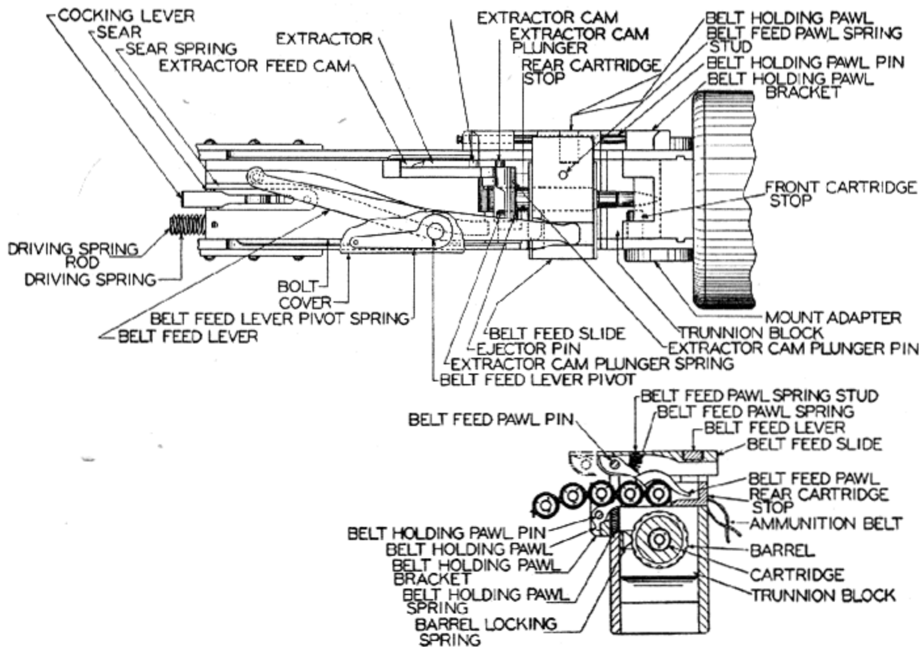
Belt-Feed Mechanism
