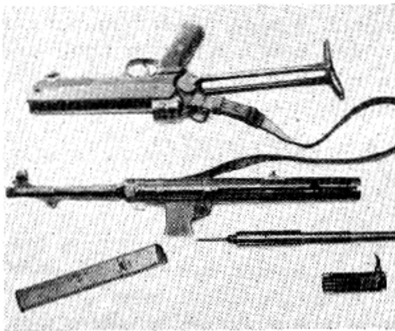
1. Weapon dismounted, complete field strip.
