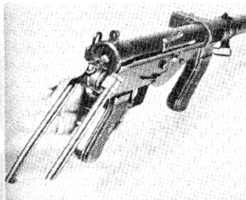
1. Push down on stock locking plunger and bend the stock down out of line with the rear of the gun.
