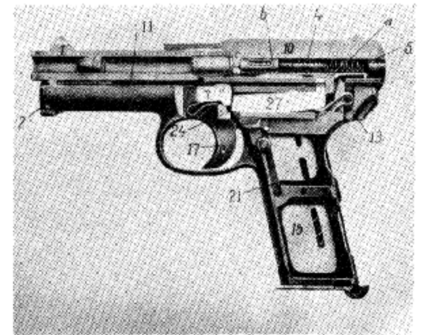
Pistol Fired, Parts Still Locked.
