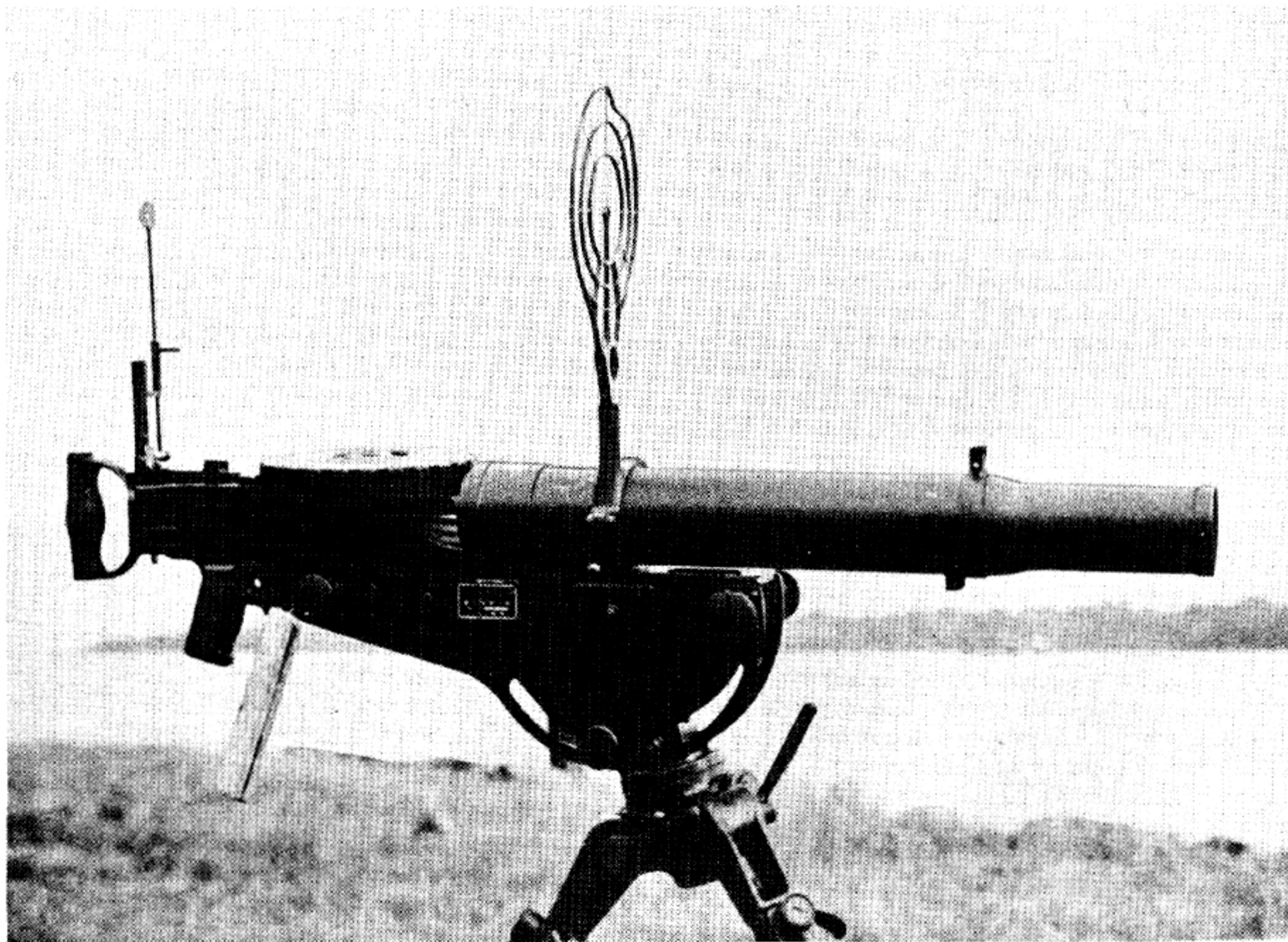
Lewis Gun Used by Japs. Special Mount and A A Sights
