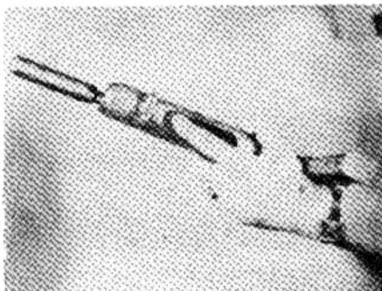
5. Now remove forefinger from Action Bar Fingerpiece and permit Action Bar to snap forward. The compressed spring will (a) Drive the Bolt forward. (b) The Bolt will push the first Cartridge into the Firing Chamber. (c) Extractor set in face of Bolt will spring over head of Cartridge and lock in groove ready to extract empty case. (d) Bolt will lock and Firing Mechanism engage so that a pressure on the Trigger will fire the Gun.
