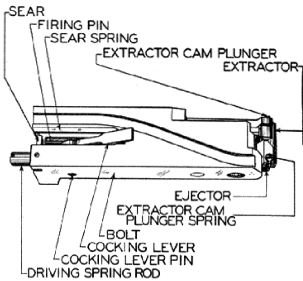
Bolt Assembly
