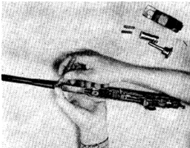
7. With left thumb, push Action Bar to rear until the dismounting hole in the Action Bar Spring Guide can be seen. Then insert end of Hammer Spring in the dismounting hole.
